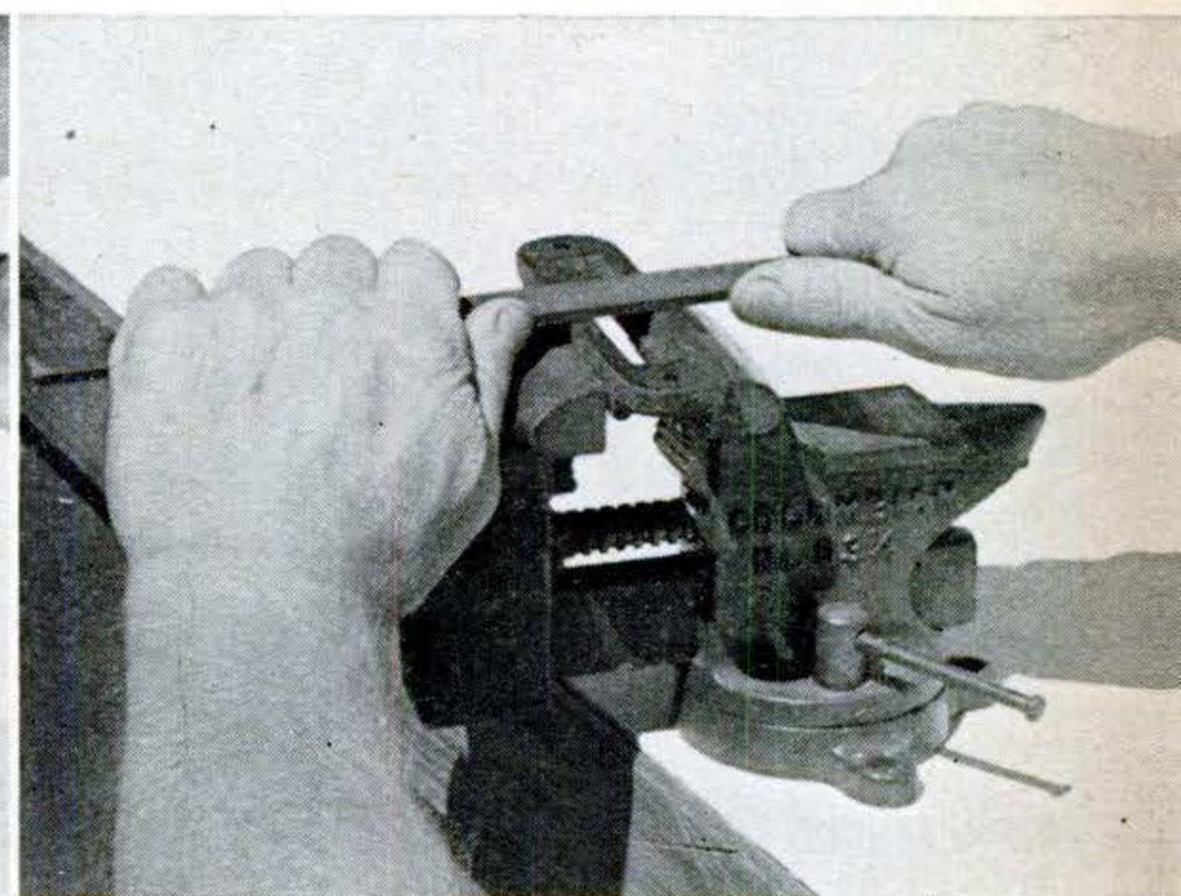
DRAWFILING , done with a mill bastard, is the way to a finer finish. The two-hand grip, with thumbs behind the file, guides it back and forth over the work.
